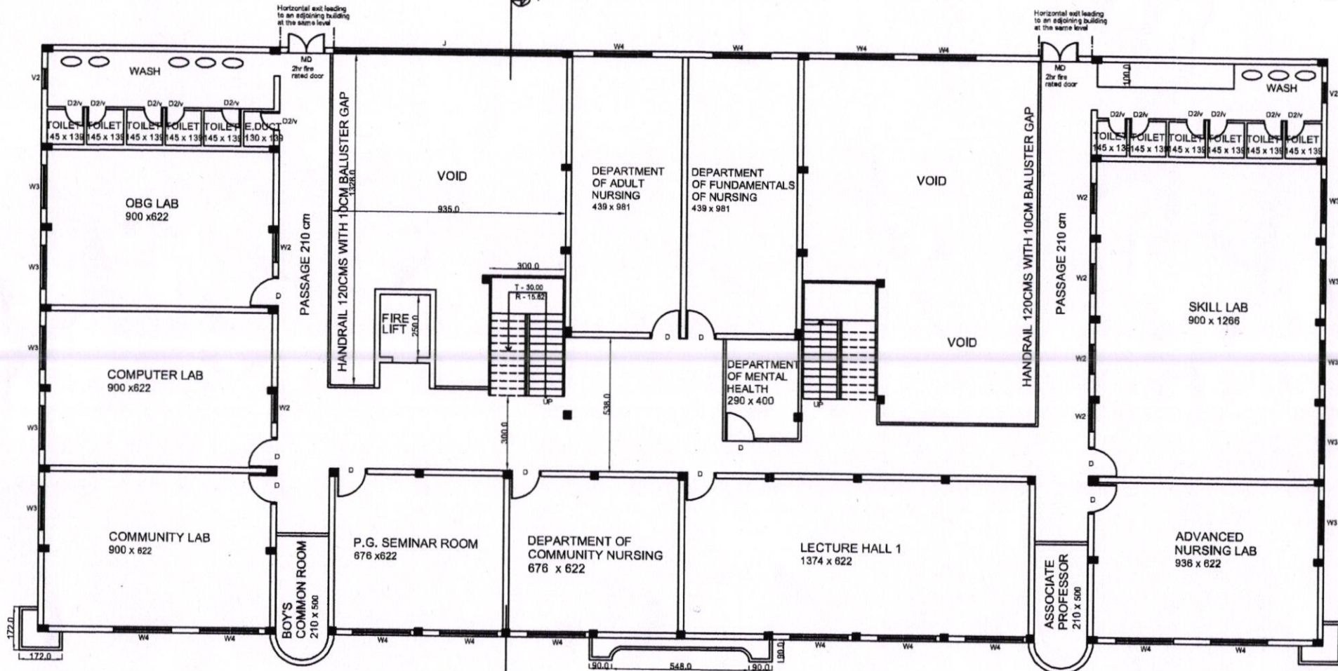
FIRST FLOOR PLAN PLINTH AREA - 943 m 2
