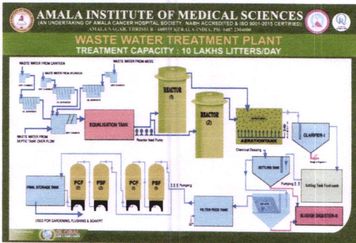
Flow diagram depicting the process of waste water treatment plant
