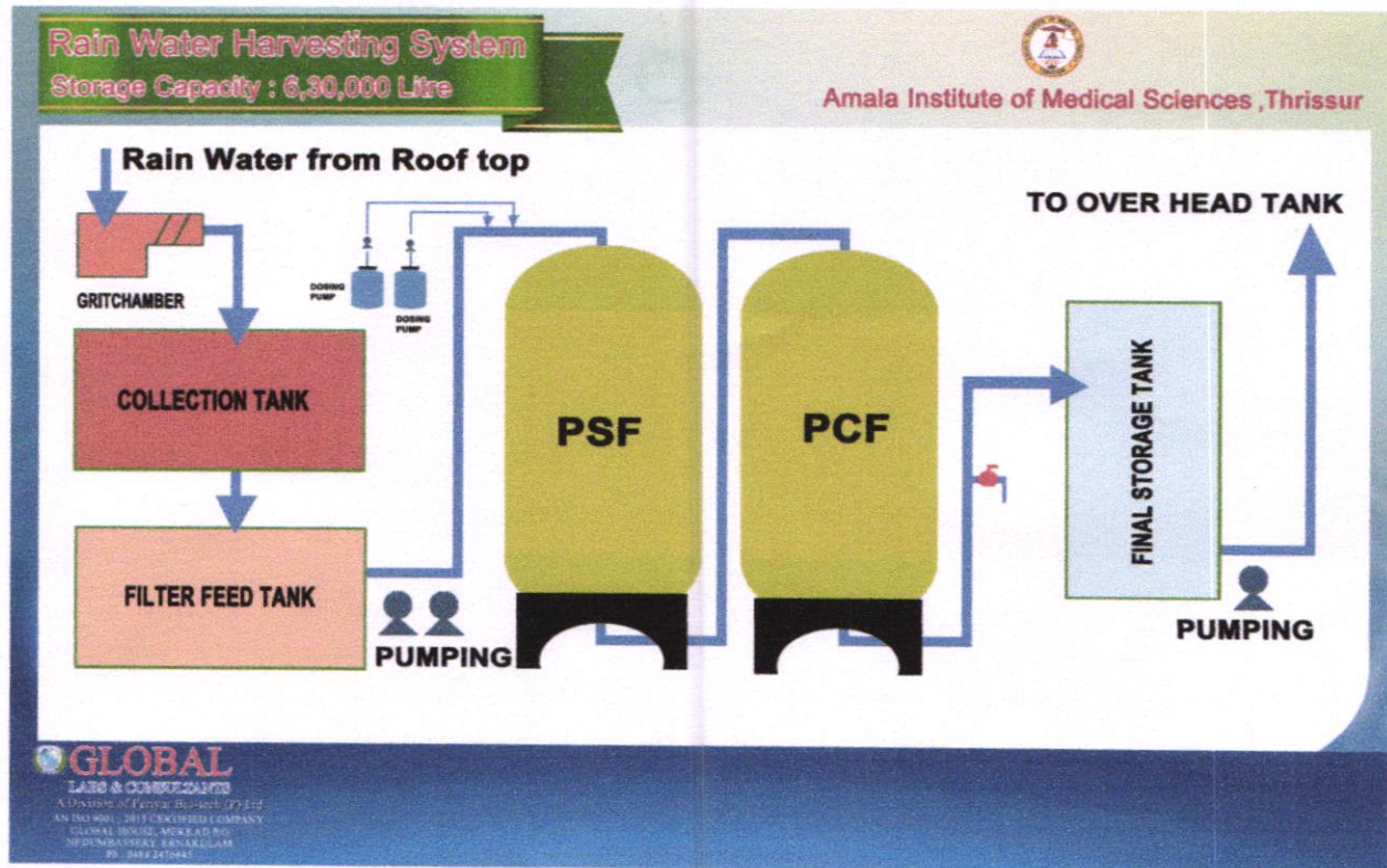
Flow diagram depicting the process of Rain water harvesting
