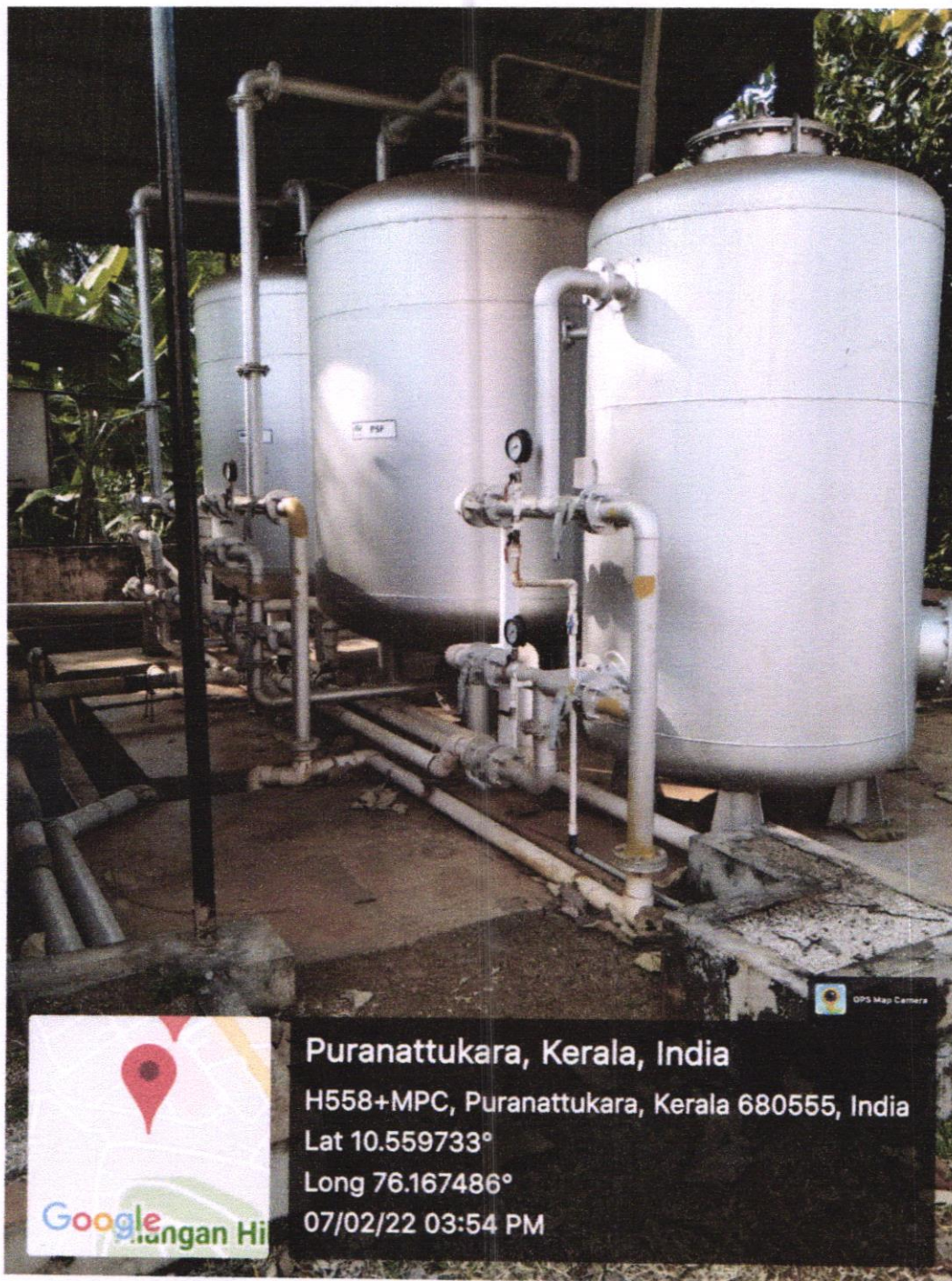
ACON, filter feed tank, rain water harvesting system
